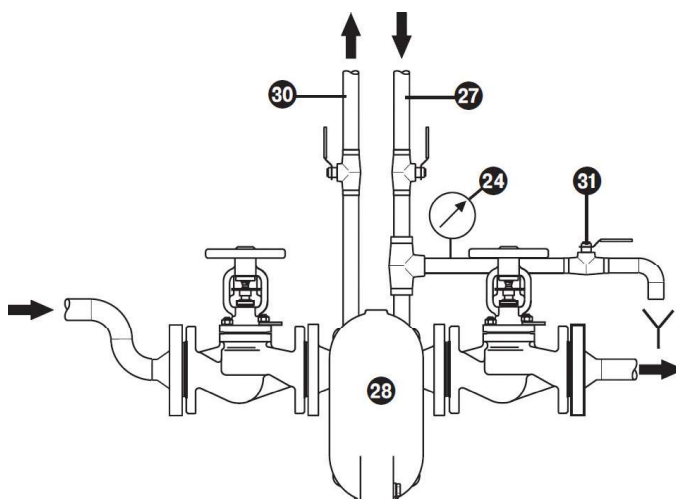
Connection of UNA 25-PS (deaeration to atmosphere)
