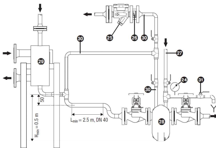
Connection of UNA 25-PK to a heat exchanger
